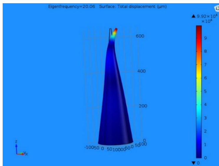
Figure 10. Displacement at mediocre stages of deformation. Source: Author.
