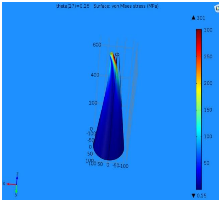
Figure 14. Stress observed at 0.25 degree. Source: Author.
