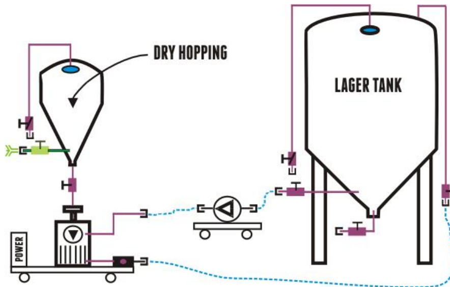
Figure 5. Rolec-DryHOPNIK System.
