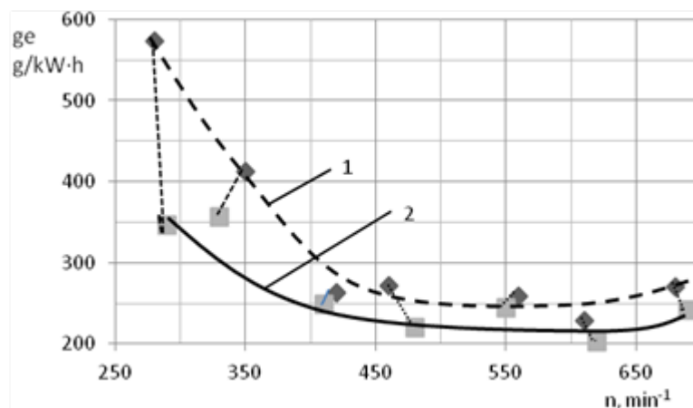
Figure 6. Specific effective diesel fuel consumption: 1 - with standard pistons; 2 - with corundum pistons Source: Authors
