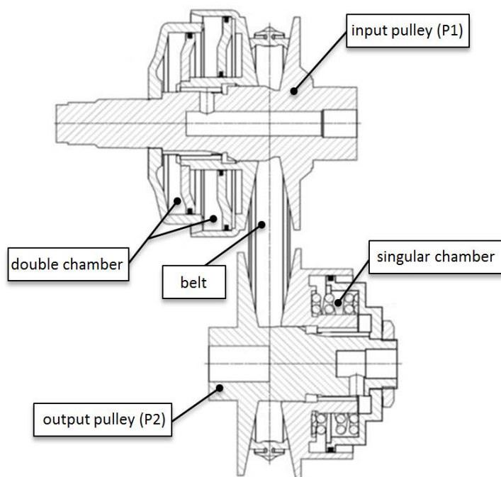
Fig. 3. Cross section of CVT
