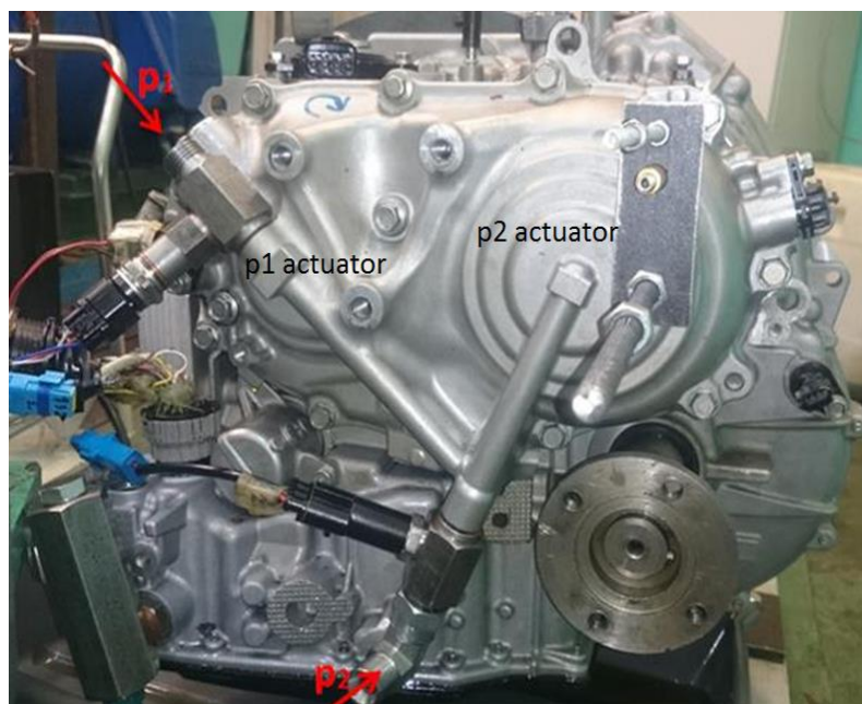
Fig. 1. Picture of the tested gearbox Source: Author's
